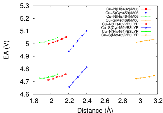
Figure 3: The value of electron affinity as a function of bond distance in T1Cu of MCOs protein. The equilibrium distance is represented by middle point with increment point 0.05 \text{ \AA} .
