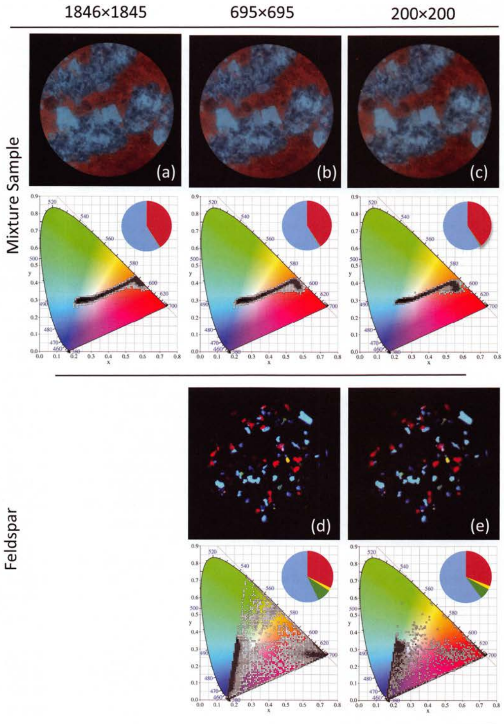
Fig. 4 Results of TLCI analysis with BP excluded type for the mixture sample (quartz and calcite) and feldspar. The class boundary values used to set the plot colors were 1, 0.1, 0.05, 0.01 and 0.001%. For mixture sample, file size is (a) 1846×1845, (b) 695×695 and (c) 200×200. For feldspar, (d) 695×695 and (e) 200×200. Circles show the proportion of each color. Each color comes from the corresponding color zone.
