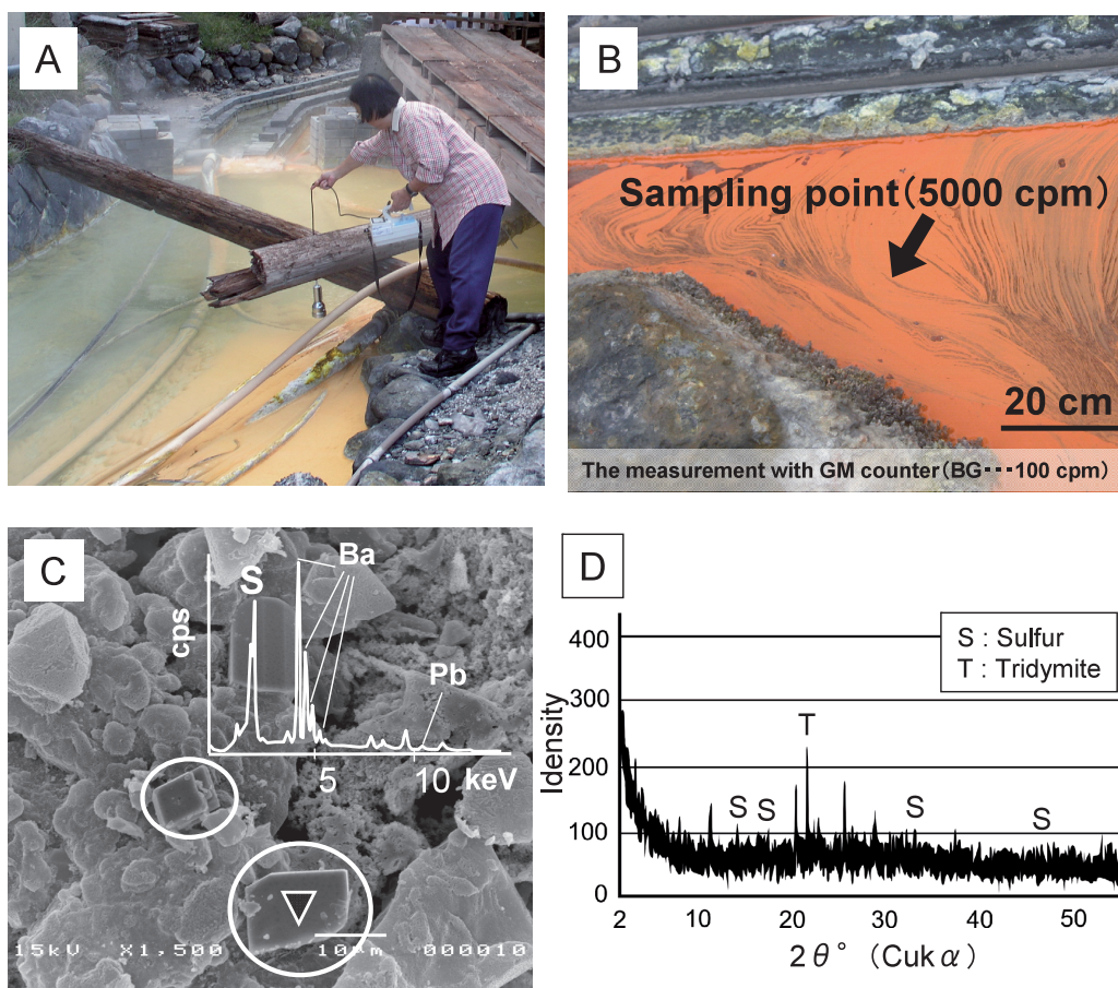
Fig. 2. Reddish brown microbial mats (A, B), the SEM-EDX micrograph of Hokutolite (C) and the XRD pattern (D) in the microbial mats collected from Tamagawa Hot Springs.
