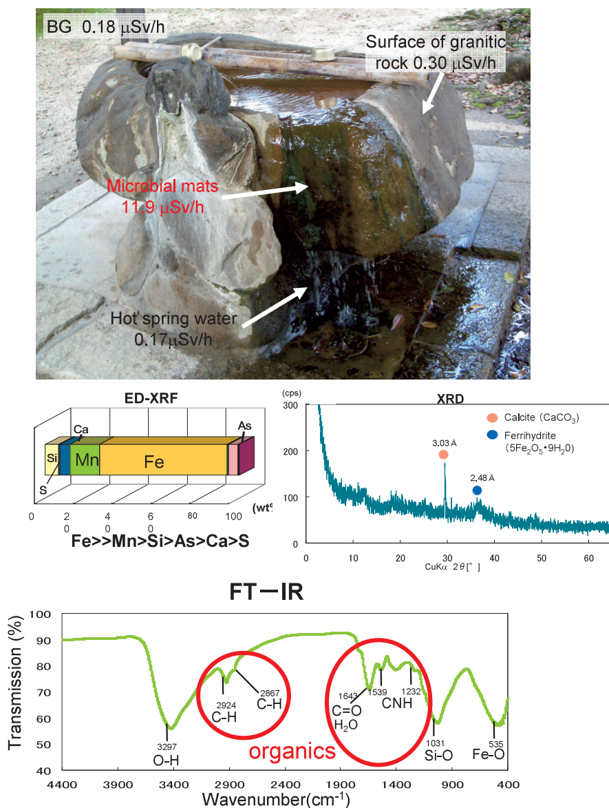
Fig. 5. Sampling points at Misasa Hot Springs in Tottori Prefecture in Japan, showing higher radioactivity of the green and reddish brown microbial mats (11.9 \mu\text{Sv/h} ; an arrow in centre) than that of hot spring water (0.17 \mu\text{Sv/h} ; an arrow in bottom), granite (0.30 \mu\text{Sv/h} ), and back ground in the air (0.18 \mu\text{Sv/h} ; BG). Energy dispersive X-ray fluorescence analysis (ED-XRF) of the microbial mats showed Mn and Fe- rich compositions (center left). X-ray powder diffraction analysis (XRD) of the microbial mats shows mainly ferrihydrite and calcite minerals (center right). Fourier transform-infrared absorbance spectroscopy (FT-TR) of the microbial mats showed rich in organics (circles)(bottom).
